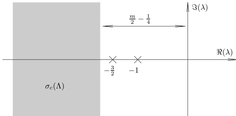
Fig. 1: The spectrum of the linear operator \Lambda in \mathbb{L}^2(m) , when m = 4 .
