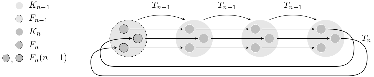
Figure 4: Two successive towers in the construction of K
