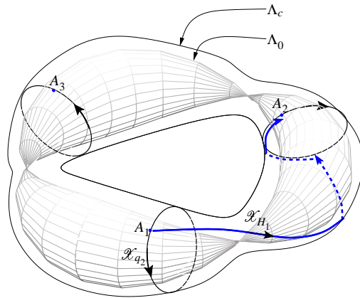
Figure 3: The multi-pinched torus
