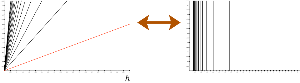
Figure 1: Allowed values for the parameters (\hbar, E) or (h, \epsilon) .
