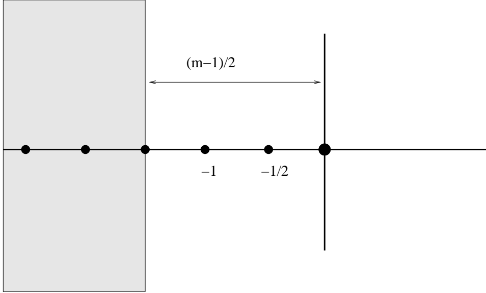
Figure 3: The spectrum of the operator \mathcal{L} on the space L^2(m) with eigenvalues at the non-positive half integers and a half plane of essential spectrum. (In the illustration, m = 4 .)
