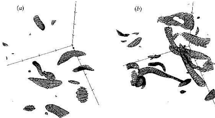
Figure 2: Plots of vorticity contours in a numerical simulation of a three-dimensional turbulent flow showing the presence of vortex tubes in the flow. (Reprint of Figure 6 with permission from Jimenez, et al. J. Fluid Mech. vol. 255, p. 65 (1993) Copyright (1993) by the Cambridge University Press.)[7]
