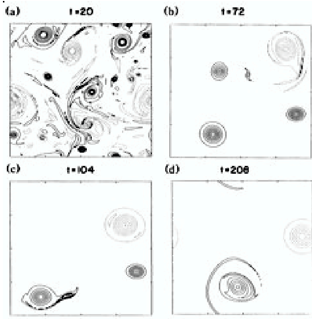
Figure 1: Plots of the iso-vorticity contours in a numerical simulation of a two-dimensional turbulent flow as a function of time. (Reprint of Figure 3 with permission from W. H. Matthaeus, et al. Phys. Rev. Lett., vol. 66, 2731 (1991), Copyright (1991) by the American Physical Society.)[9]
