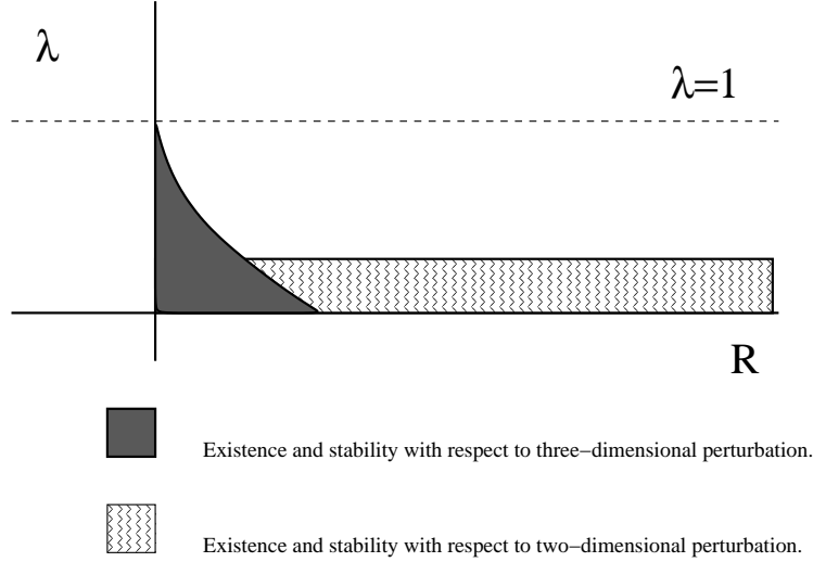
Figure 4: An illustration of the regions in which we can prove the existence of non-axisymmetric Burgers vortices
