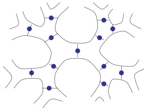
Figure 1. D^* and its canonical rigid structure.
